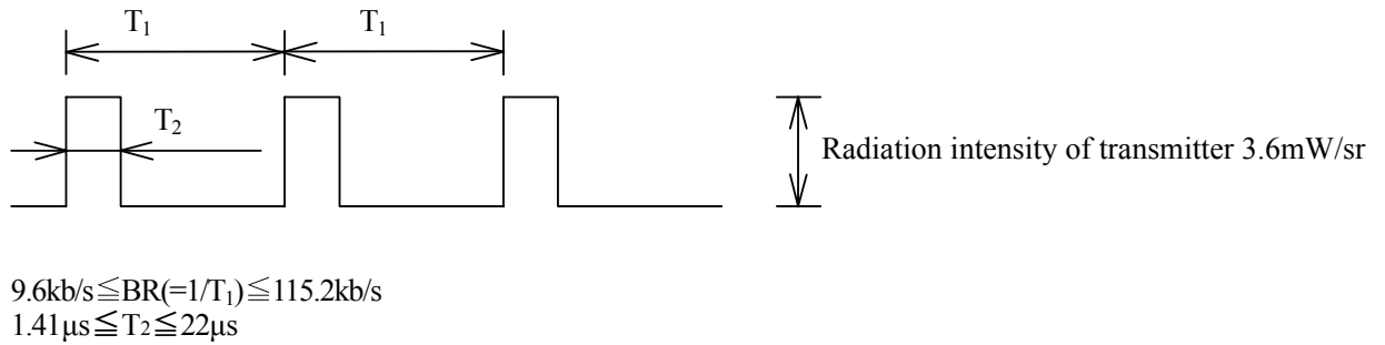
Fig.2 Input Signal Waveform(Receiver side)
